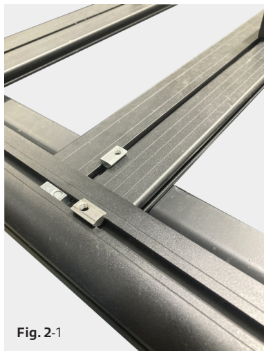
Fig. 2-1 Placement of slot nuts
