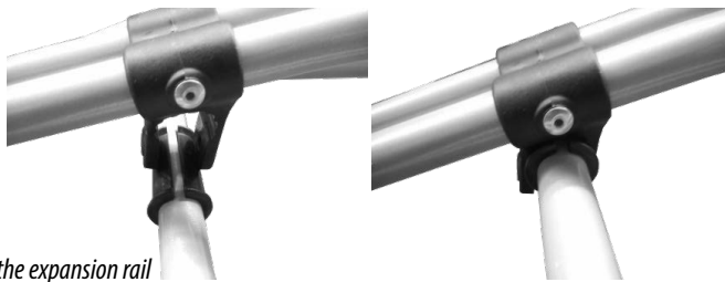
Figures 6 and 7: Position the expansion rail
