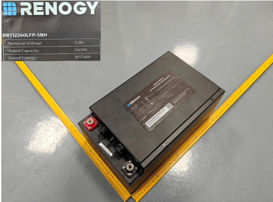
Battery / 电池组 (RBT12240LFP-SBH 12.8V 240Ah 3072Wh)
